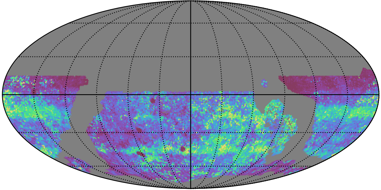
ddf_acor_sf20_lsf40_lsr50_v3.4_10yrs WFD zy bands: 75th Percentile Intranight Timespan
