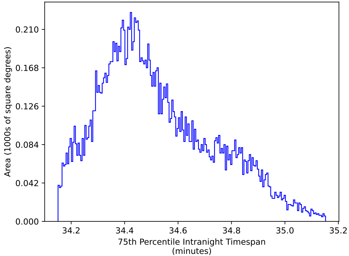
ddf_acor_sf20_ls40_lsr50_v3.4_10yrs WFD zy bands: 75th Percentile Intranight Timespan
