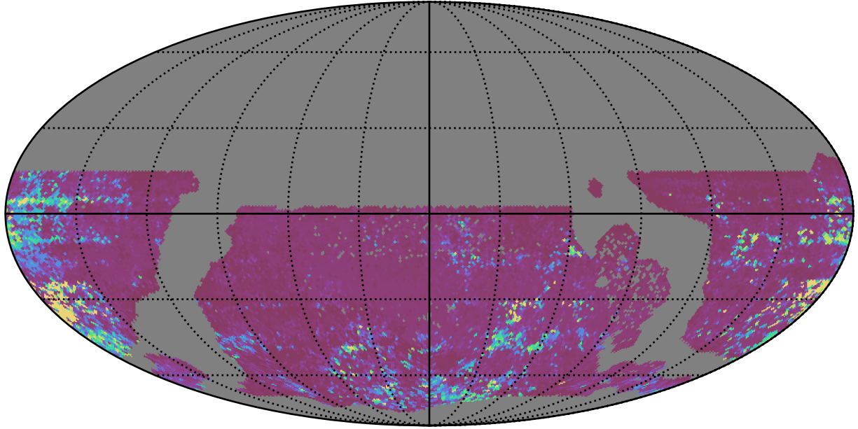
ddf_acor_sf20_lsf40_lsr50_v3.4_10yrs WFD z band: 75th Percentile Intranight Timespan
