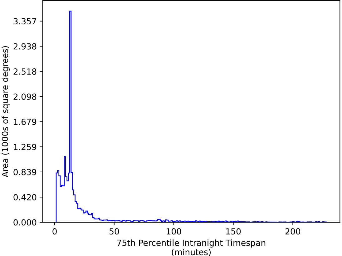
ddf_acor_sf20_lsf40_lsr50_v3.4_10yrs WFD z band: 75th Percentile Intranight Timespan
