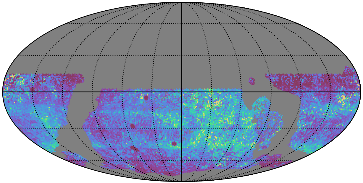
ddf_acor_sf20_lsf40_lsr50_v3.4_10yrs WFD y band: 75th Percentile Intranight Timespan
