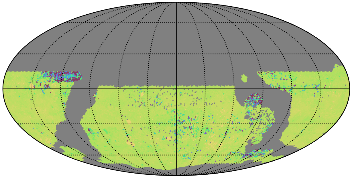
ddf_acor_sf20_lsf40_lsr50_v3.4_10yrs WFD ug bands: 75th Percentile Intranight Timespan
