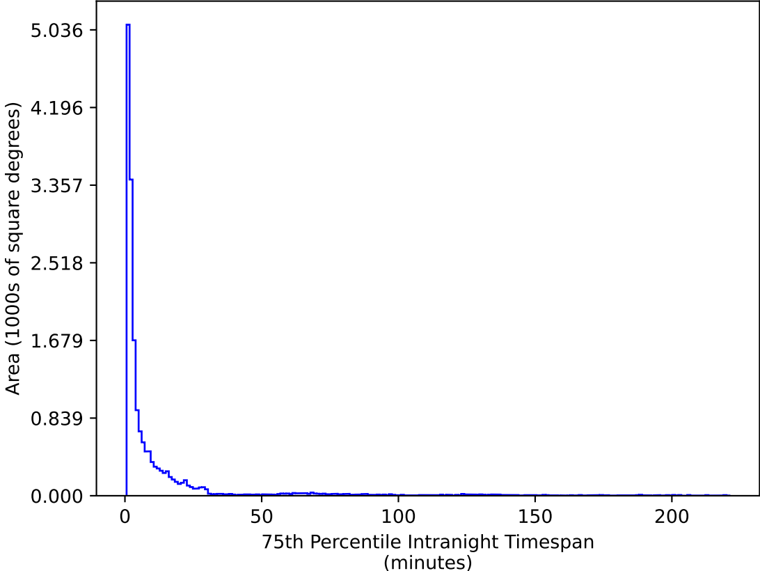
ddf_acor_sf20_lsf40_lsr50_v3.4_10yrs WFD u band: 75th Percentile Intranight Timespan
