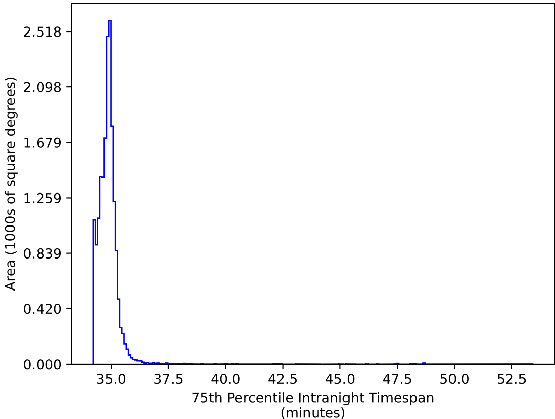
ddf_acor_sf20_lsf40_lsr50_v3.4_10yrs WFD iz bands: 75th Percentile Intranight Timespan
