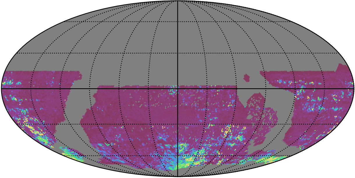
ddf_acor_sf20_lsf40_lsr50_v3.4_10yrs WFD i band: 75th Percentile Intranight Timespan
