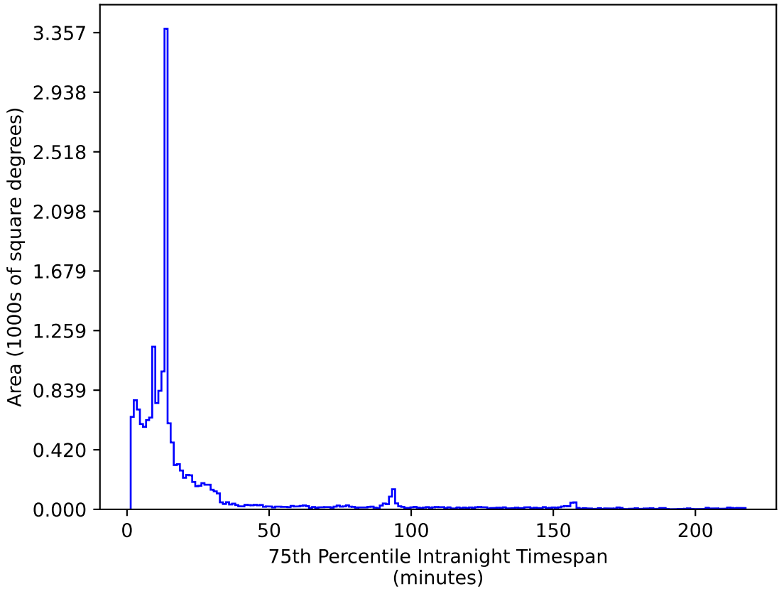
ddf_acor_sf20_lsf40_lsr50_v3.4_10yrs WFD i band: 75th Percentile Intranight Timespan
