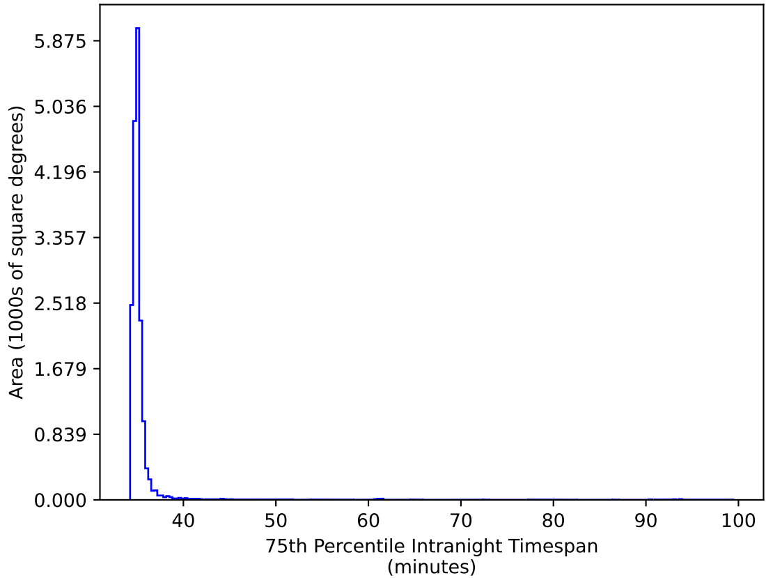
ddf_acor_sf20_lsf40_lsr50_v3.4_10yrs WFD gr bands: 75th Percentile Intranight Timespan
