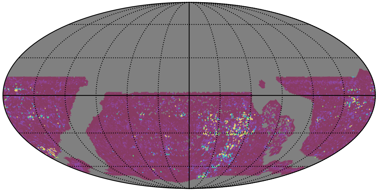
ddf_acor_sf20_lsf40_lsr50_v3.4_10yrs WFD g band: 75th Percentile Intranight Timespan
