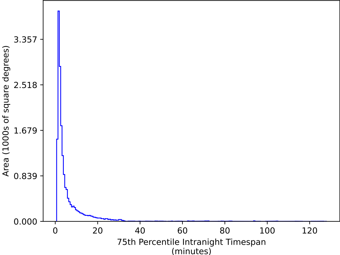
ddf_acor_sf20_lsf40_lsr50_v3.4_10yrs WFD g band: 75th Percentile Intranight Timespan
