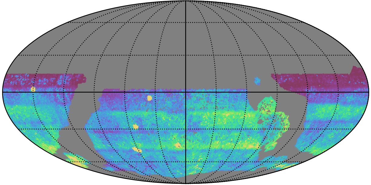
ddf_acor_sf20_lsf40_lsr50_v3.4_10yrs WFD all bands: 75th Percentile Intranight Timespan
