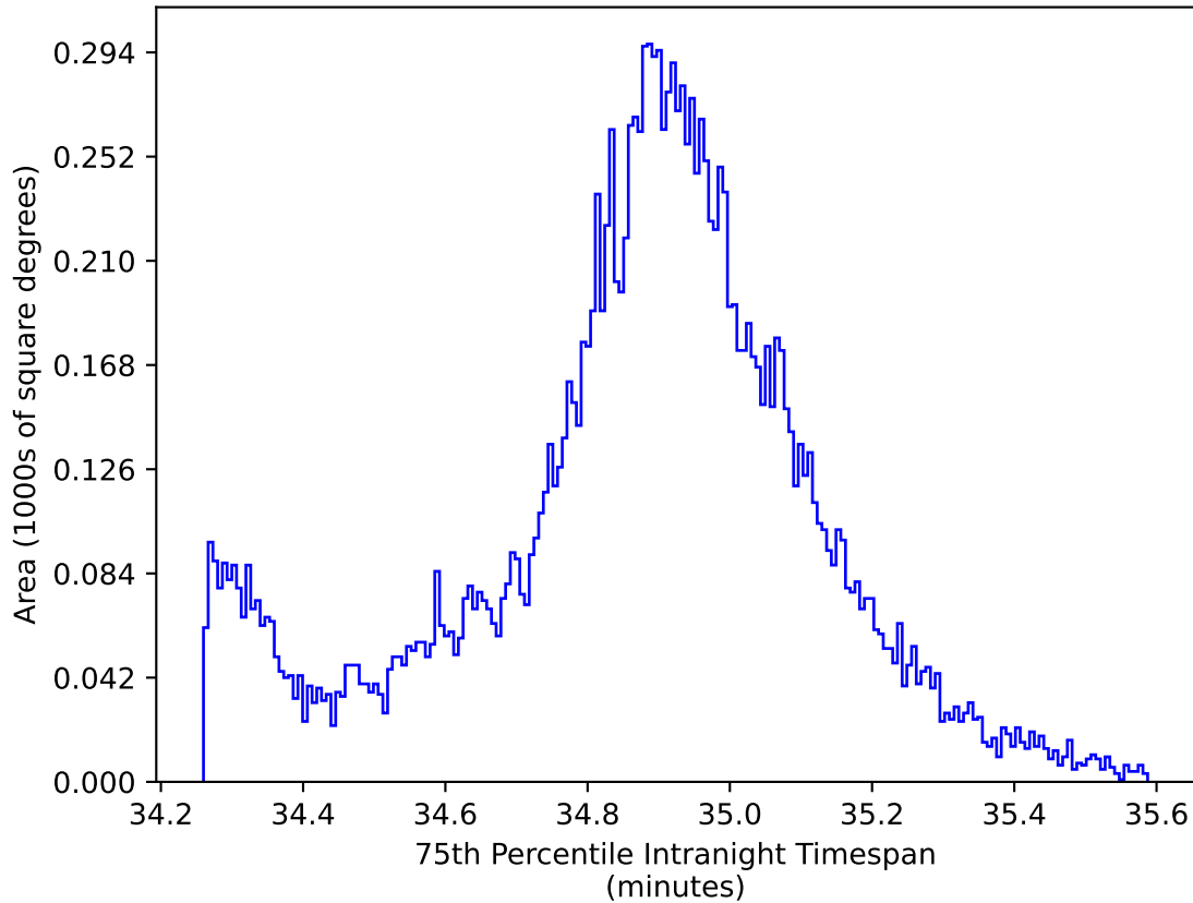
ddf_acor_sf20_Isf40_Isr50_v3.4_10yrs WFD all bands: 75th Percentile Intranight Timespan
