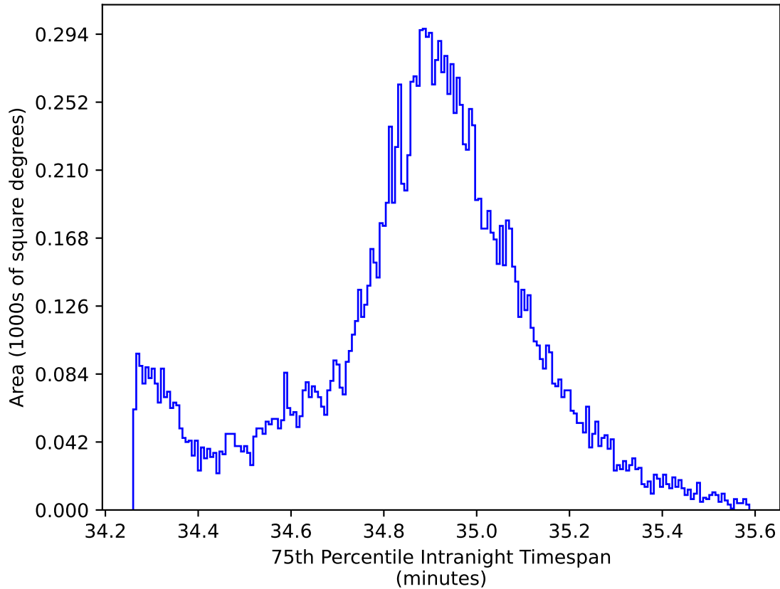
ddf_acor_sf20_lsf40_lsr50_v3.4_10yrs WFD: 75th Percentile Intranight Timespan
