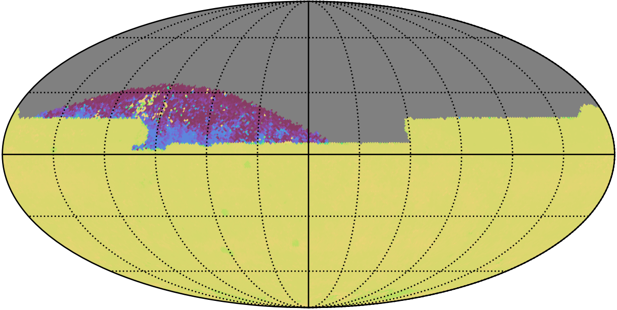
ddf_acor_sf20_lsf40_lsr50_v3.4_10yrs All sky zy bands: 75th Percentile Intranight Timespan
