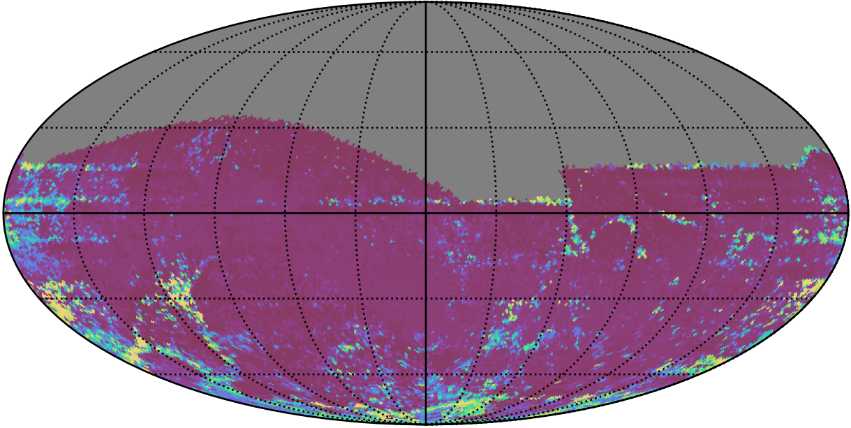
ddf_acor_sf20_lsf40_lsr50_v3.4_10yrs All sky z band: 75th Percentile Intranight Timespan
