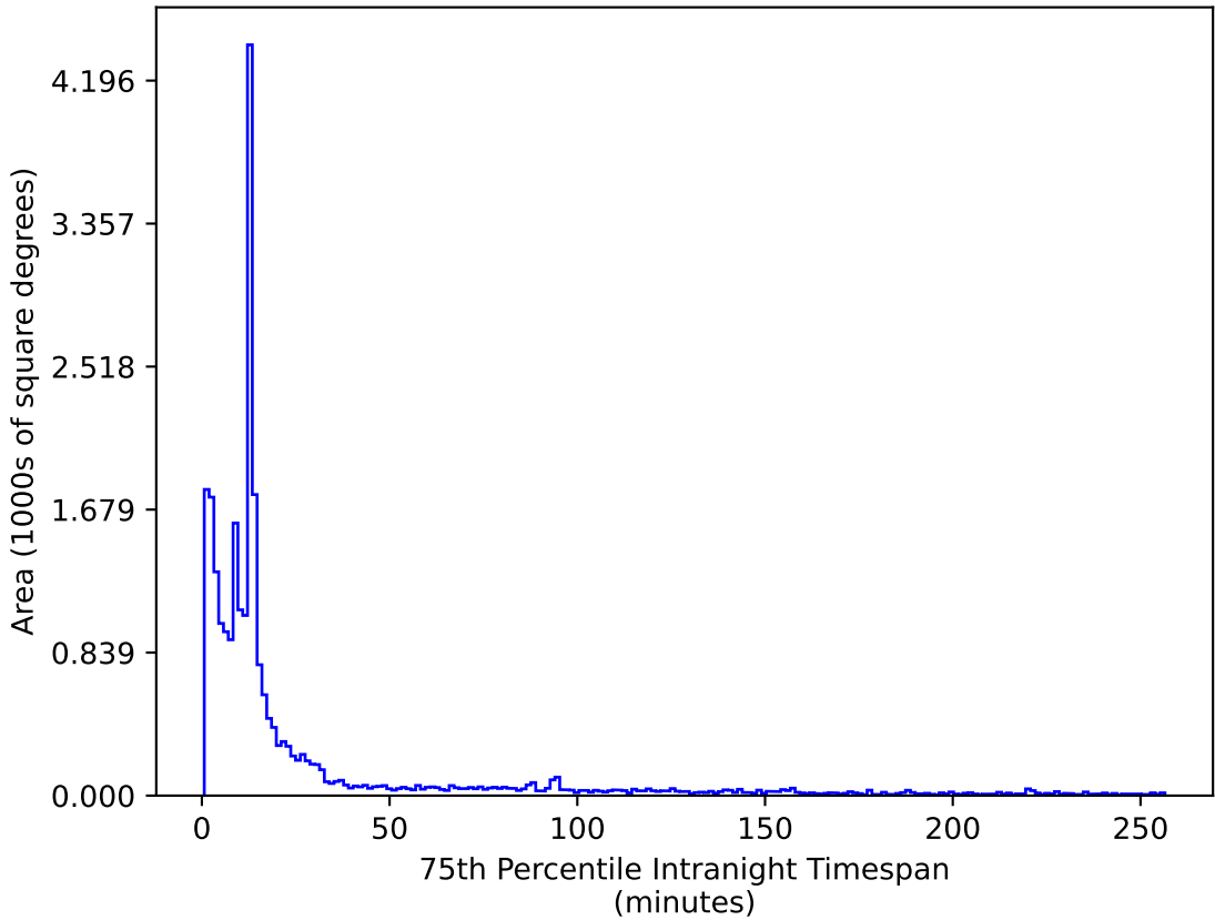
ddf_acor_sf20_lsf40_lsr50_v3.4_10yrs All sky z band: 75th Percentile Intranight Timespan
