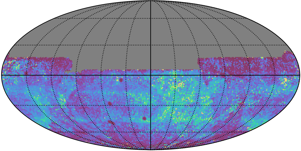
ddf_acor_sf20_lsf40_lsr50_v3.4_10yrs All sky y band: 75th Percentile Intranight Timespan
