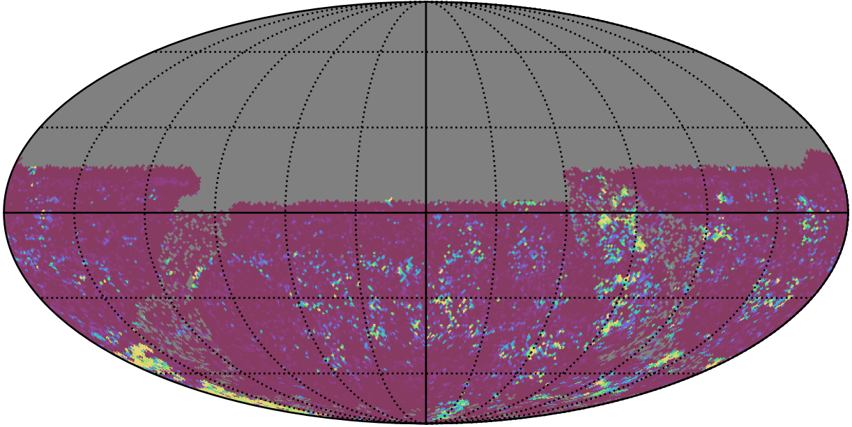
ddf_acor_sf20_lsf40_lsr50_v3.4_10yrs All sky u band: 75th Percentile Intranight Timespan
