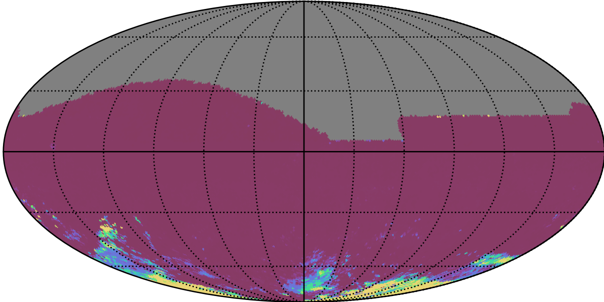
ddf_acor_sf20_lsf40_lsr50_v3.4_10yrs All sky ri bands: 75th Percentile Intranight Timespan
