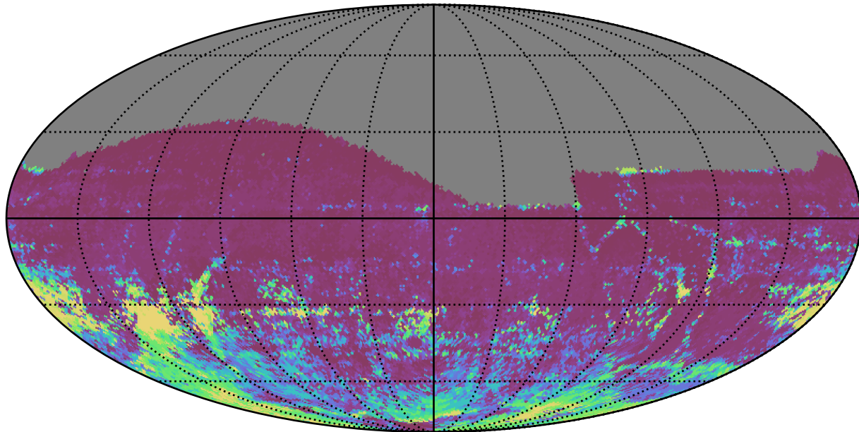
ddf_acor_sf20_lsf40_lsr50_v3.4_10yrs All sky r band: 75th Percentile Intranight Timespan
