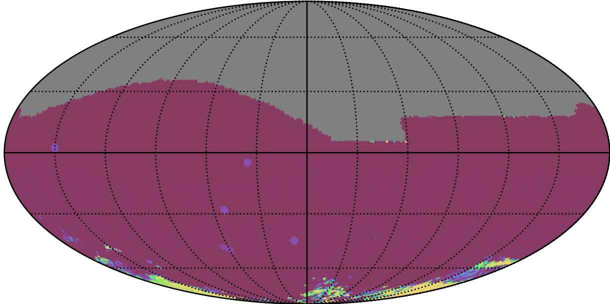
ddf_acor_sf20_lsf40_lsr50_v3.4_10yrs All sky iz bands: 75th Percentile Intranight Timespan
