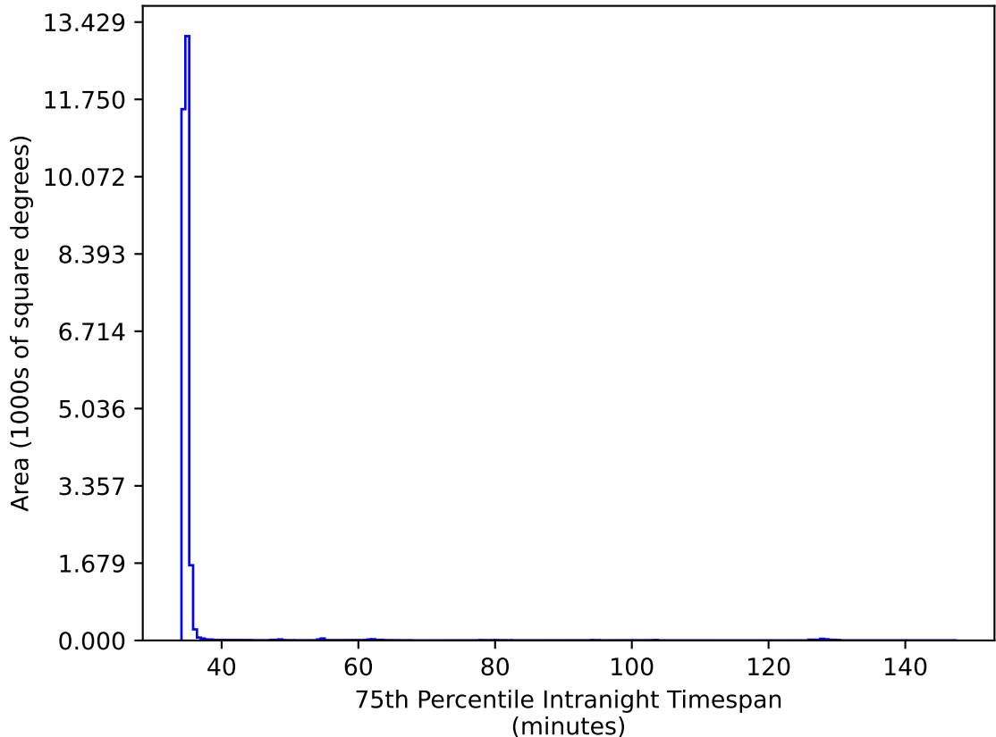
ddf_acor_sf20_lsf40_lsr50_v3.4_10yrs All sky iz bands: 75th Percentile Intranight Timespan
