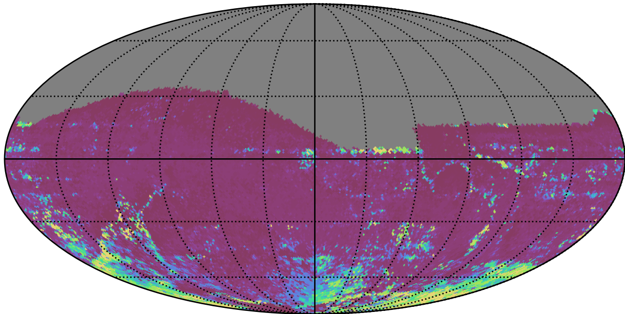
ddf_acor_sf20_lsf40_lsr50_v3.4_10yrs All sky i band: 75th Percentile Intranight Timespan
