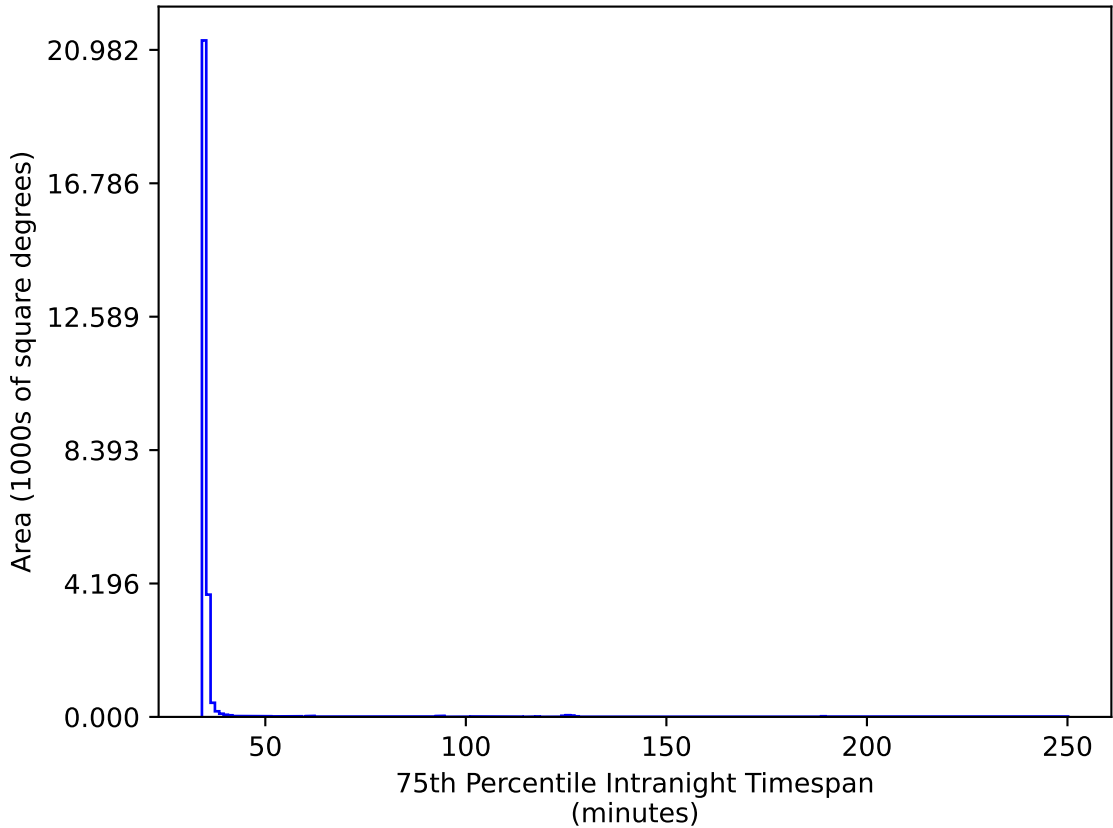
ddf_acor_sf20_lsf40_lsr50_v3.4_10yrs All sky gr bands: 75th Percentile Intranight Timespan
