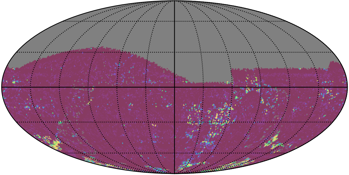
ddf_acor_sf20_lsf40_lsr50_v3.4_10yrs All sky g band: 75th Percentile Intranight Timespan
