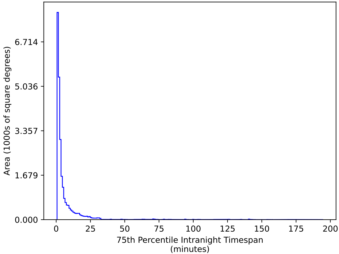
ddf_acor_sf20_lsf40_lsr50_v3.4_10yrs All sky g band: 75th Percentile Intranight Timespan
