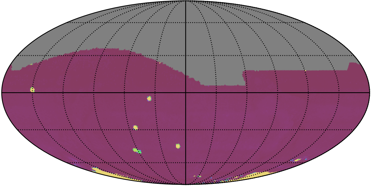
ddf_acor_sf20_lsf40_lsr50_v3.4_10yrs All sky all bands: 75th Percentile Intranight Timespan
