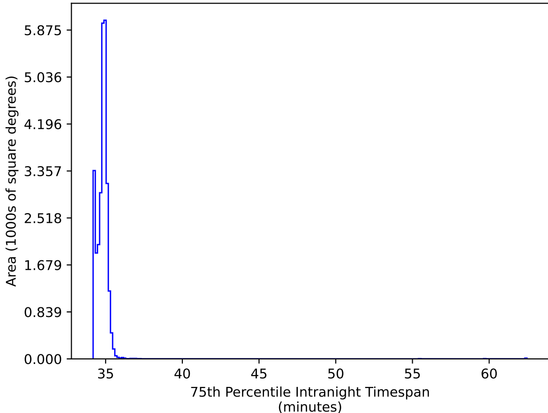
ddf_acor_sf20_lsf40_lsr50_v3.4_10yrs All sky all bands: 75th Percentile Intranight Timespan
