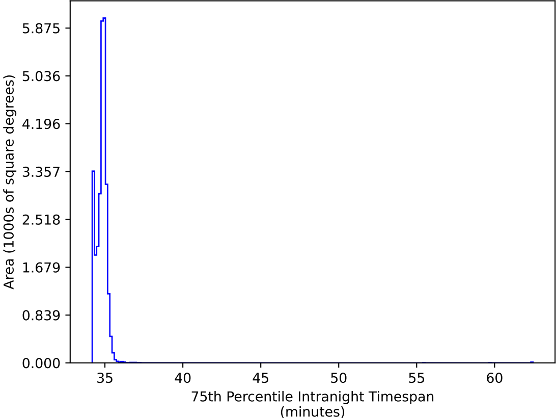
ddf_acor_sf20_lsf40_lsr50_v3.4_10yrs All sky: 75th Percentile Intranight Timespan
