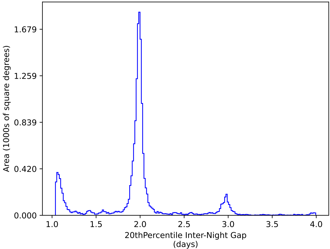
ddf_acor_sf20_lsf40_lsr50_v3.4_10yrs WFD y band: 20thPercentile Inter-Night Gap
