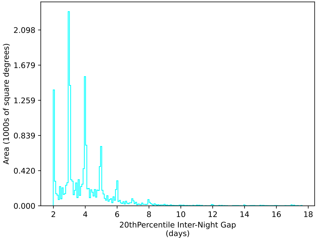
ddf_acor_sf20_ls40_lsr50_v3.4_10yrs WFD u band: 20thPercentile Inter-Night Gap
