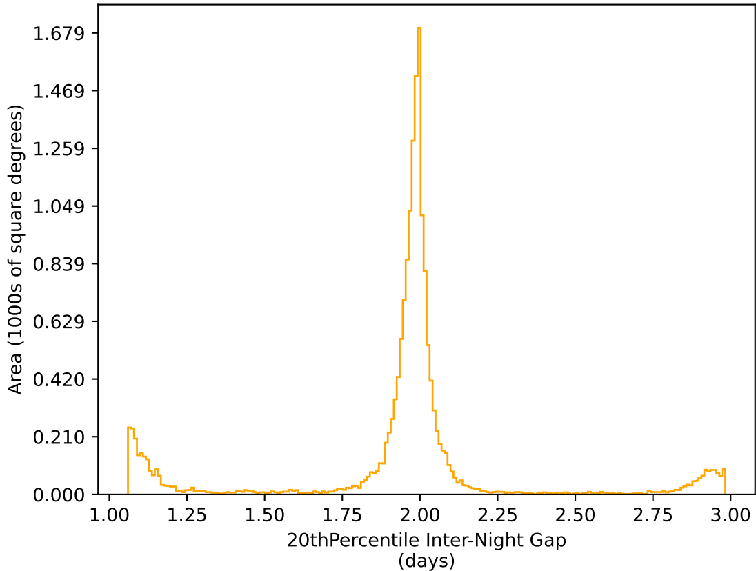
ddf_acor_sf20_lsf40_lsr50_v3.4_10yrs WFD r band: 20thPercentile Inter-Night Gap
