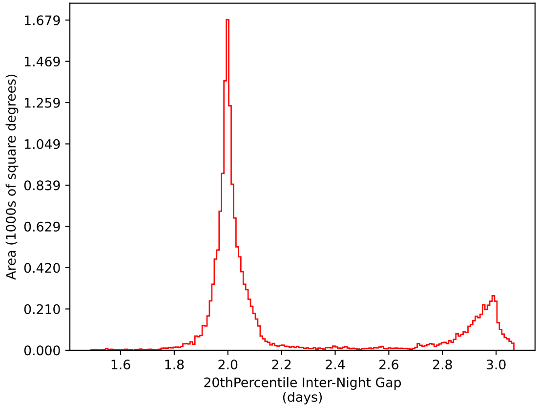
ddf_acor_sf20_lsf40_lsr50_v3.4_10yrs WFD i band: 20thPercentile Inter-Night Gap
