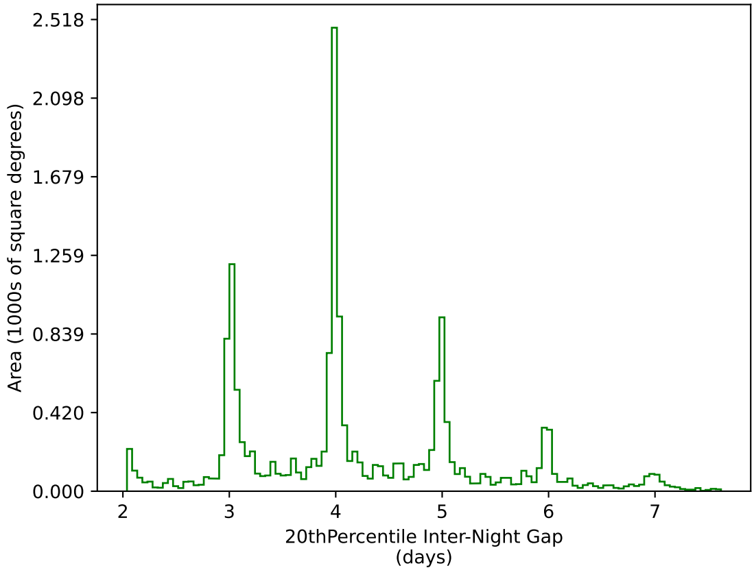
ddf_acor_sf20_lsf40_lsr50_v3.4_10yrs WFD g band: 20thPercentile Inter-Night Gap
