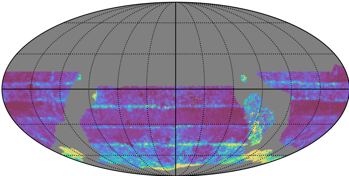
ddf_acor_sf20_lsf40_lsr50_v3.4_10yrs WFD all bands: 20thPercentile Inter-Night Gap
