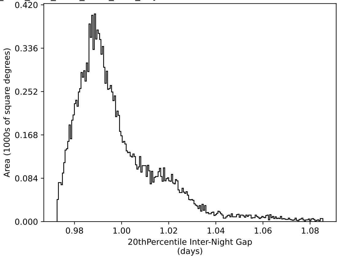
ddf_acor_sf20_ls40_lsr50_v3.4_10yrs WFD all bands: 20thPercentile Inter-Night Gap
