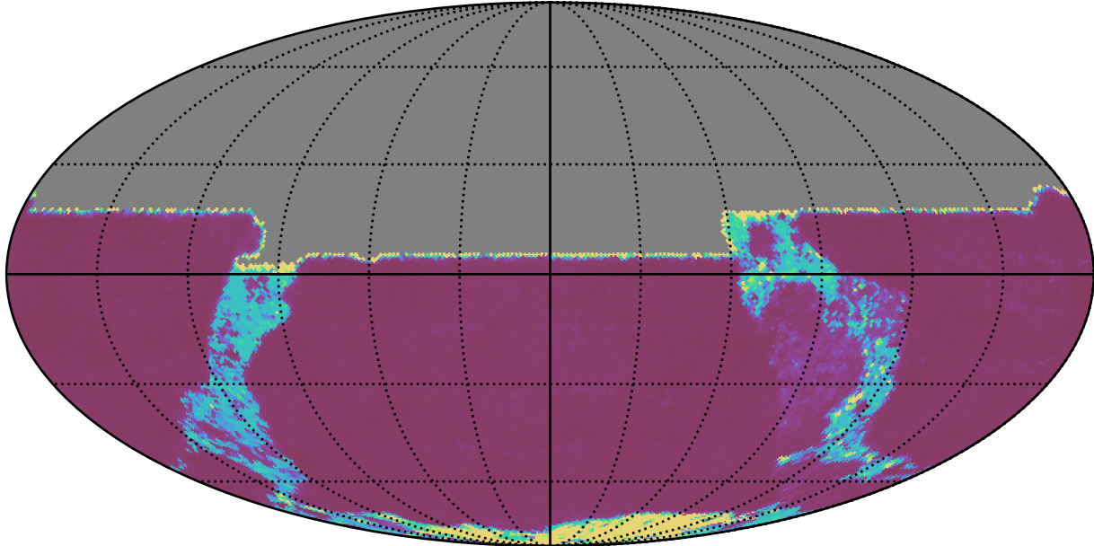
ddf_acor_sf20_lsf40_lsr50_v3.4_10yrs All sky y band: 20thPercentile Inter-Night Gap
