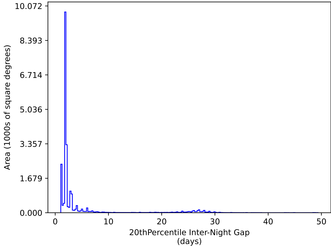
ddf_acor_sf20_ls40_lsr50_v3.4_10yrs All sky y band: 20thPercentile Inter-Night Gap
