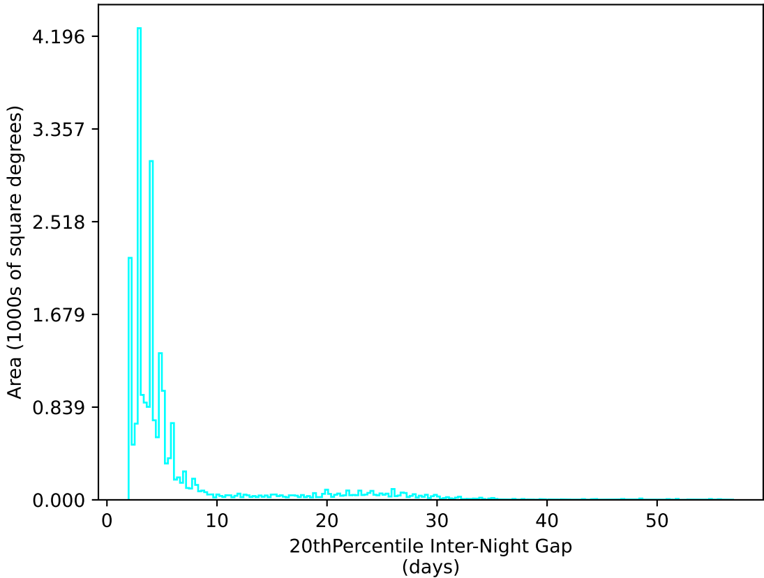
ddf_acor_sf20_lsf40_lsr50_v3.4_10yrs All sky u band: 20thPercentile Inter-Night Gap
