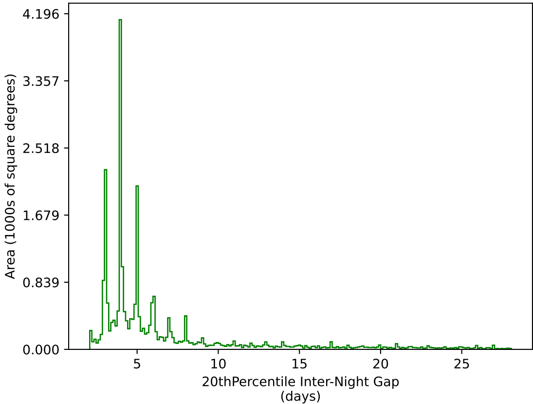
ddf_acor_sf20_lsf40_lsr50_v3.4_10yrs All sky g band: 20thPercentile Inter-Night Gap
