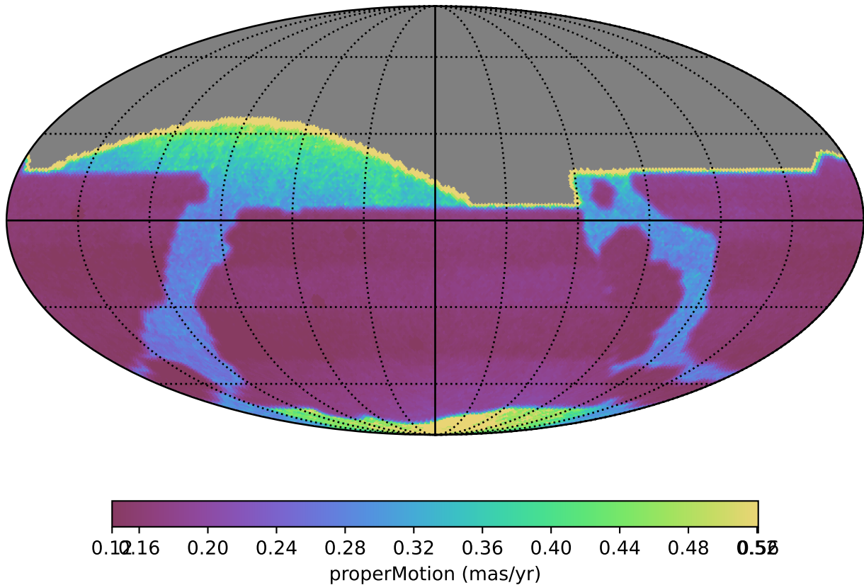
ddf_acor_sf20_lsf40_lsr50_v3.4_10yrs : properMotion
