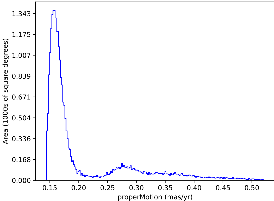
ddf_acor_sf20_ls40_lsr50_v3.4_10yrs : properMotion
