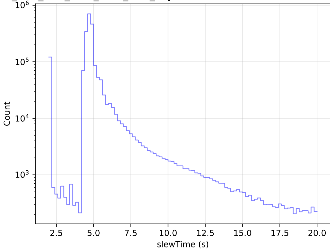
ddf_acor_sf20_Isf40_Isr50_v3.4_10yrs All visits: Zoom Slew Time Histogram
