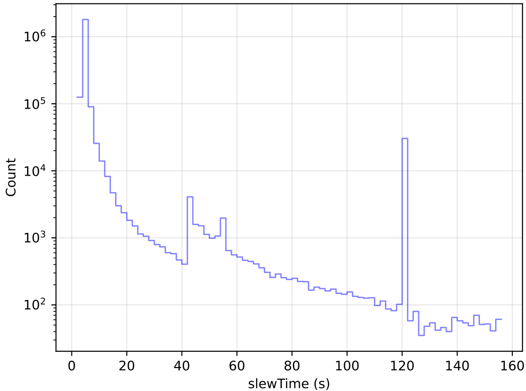
ddf_acor_sf20_lsf40_lsr50_v3.4_10yrs All visits: Slew Time Histogram
