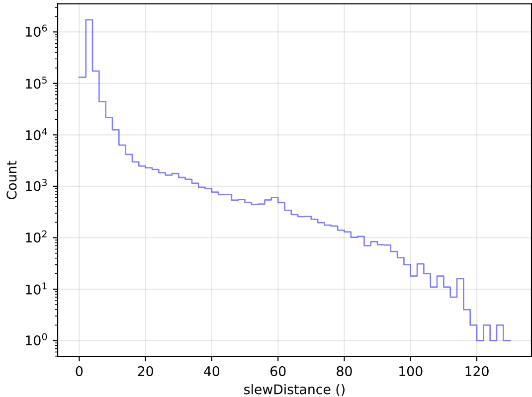
ddf_acor_sf20_lsf40_lsr50_v3.4_10yrs All visits: Slew Distance Histogram
