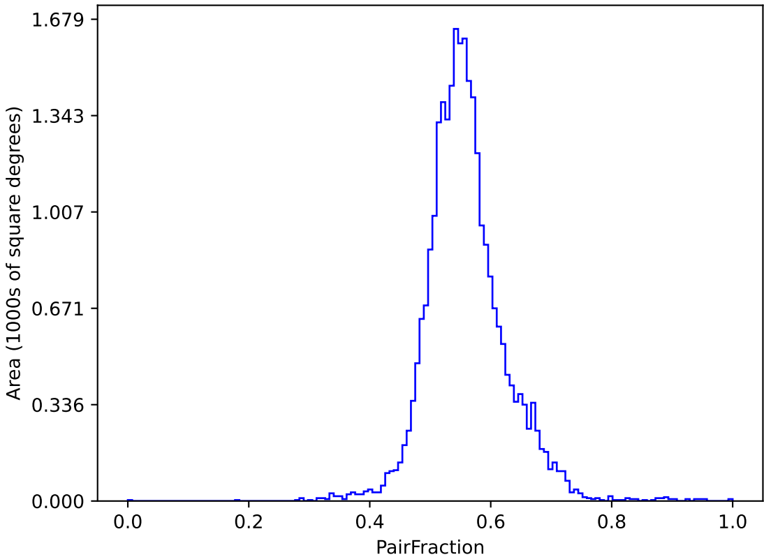
ddf_acor_sf20_lsf40_lsr50_v3.4_10yrs (g or r or i): PairFraction
