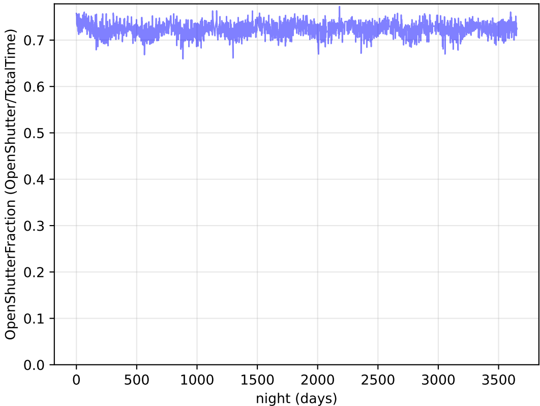
ddf_acor_sf20_lsf40_lsr50_v3.4_10yrs : OpenShutterFraction
